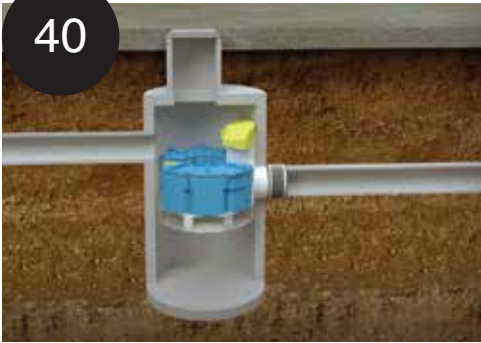
Up-Flo Filters
